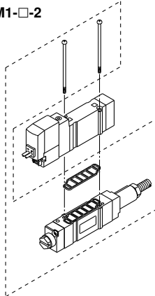
ARBY3000-M1-□-2
