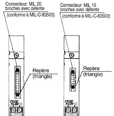
45PG (20 broches)
