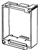
Flush Mounting Adapter (provided with H5CX-A□ models) Y92F-30
