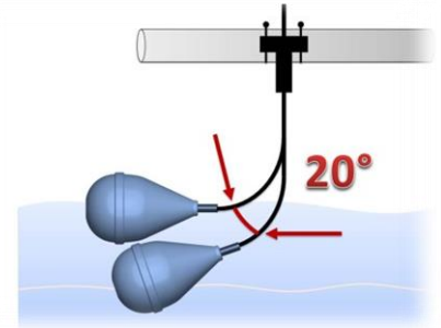
Activation angle: 20°
