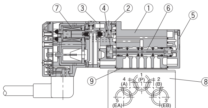
5/2 bistable
