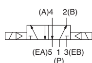
5/2 bistable
