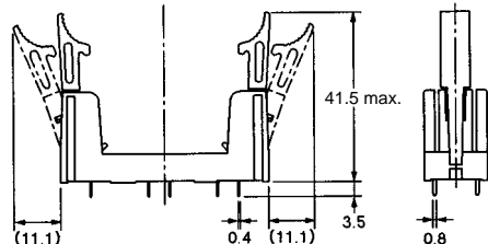
G7SA-3A1B Mounted
