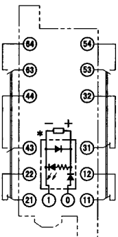
G7SA-3A3B Mounted
