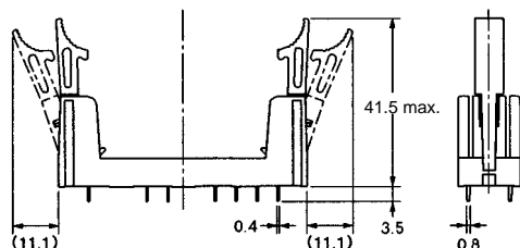
G7SA-4A2B Mounted
