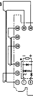
G7SA-3A1B Mounted
