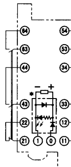
G7SA-4A2B Mounted
