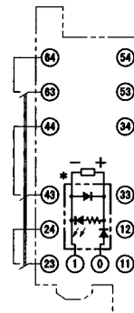
G7SA-5A1B Mounted
