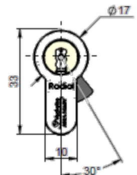
Cylindre double
