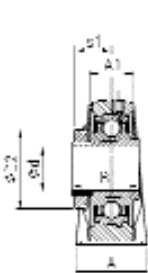
UKPE200H
