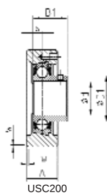
USC200
