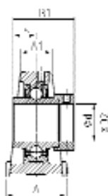
EXPAE200
