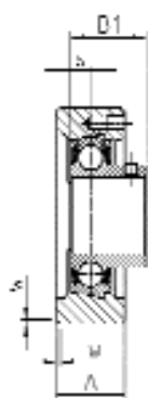
USC200
