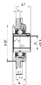
UCFS300
