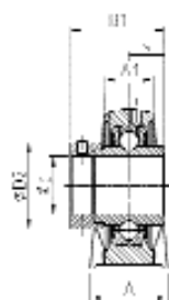
EXPE200
