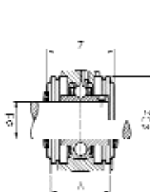
UCP200CO(CC)
